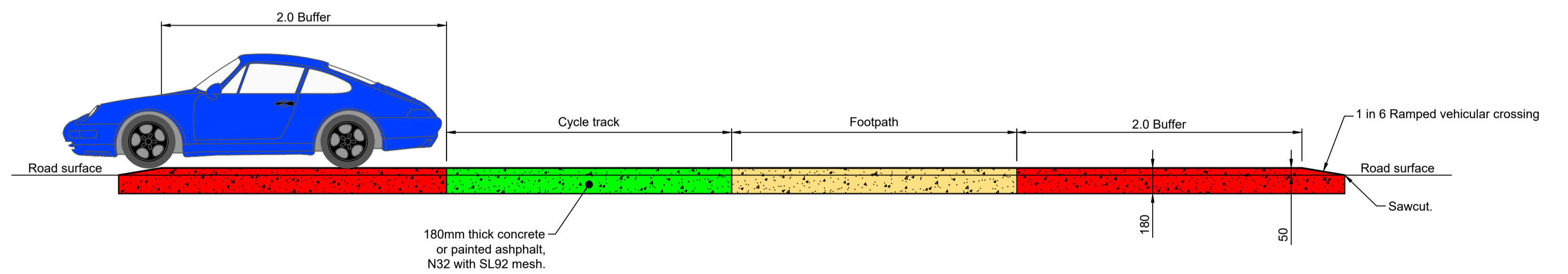
Section B-B: Road hump profile
