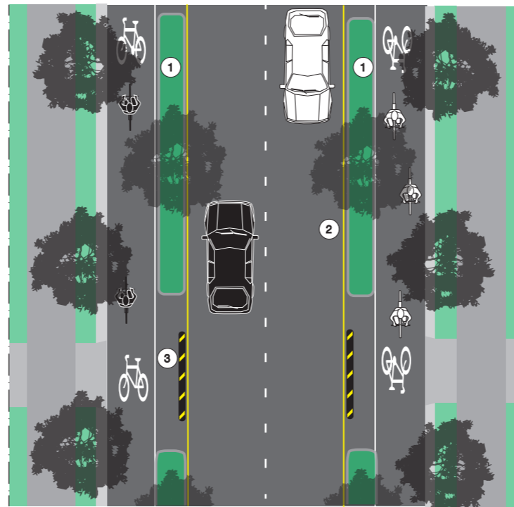
Two x 1-way separated cycle track (preferred) LTS1
