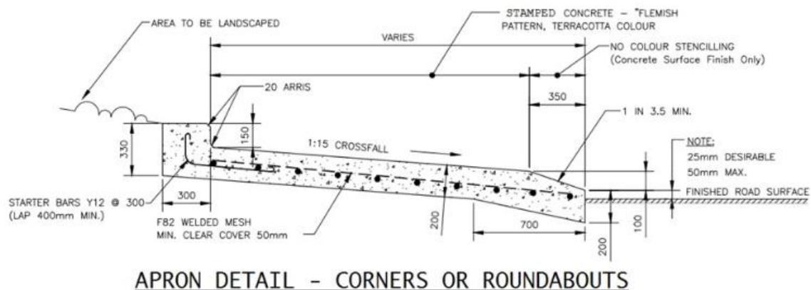
Figure 4.4(B) – Example apron detail for corners or roundabout centre island
