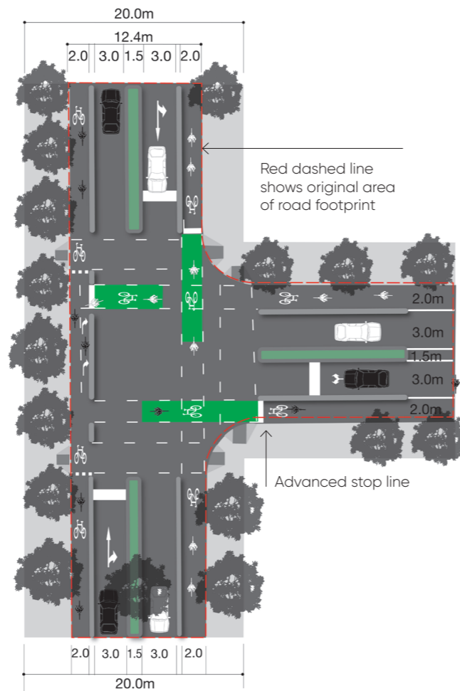
RETROFIT ADVANCE STOP LINES AND CYCLE TRACK ON APPROACHES (no kerb changes) LTS2
