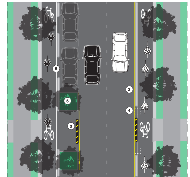
Two x 1-way separated cycle track (narrow with car parking) LTS1
