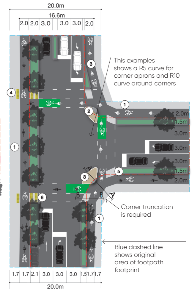
RETROFIT PROTECTED INTERSECTION (kerb changes and corner truncation) LTS1
