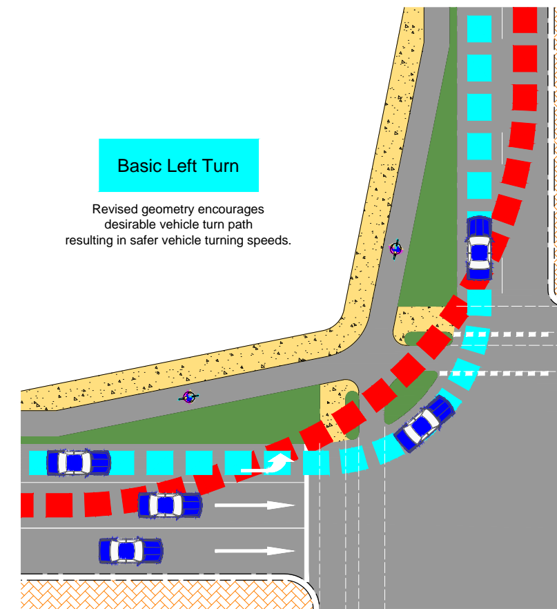
Basic left turn showing low speed vehicle travel path
