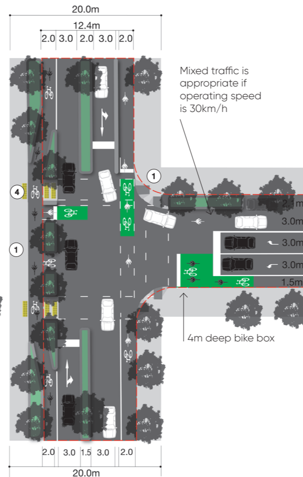
RETROFIT PARTIAL PROTECTED INTERSECTION (some kerb changes, bike box on minor road) LTS2
