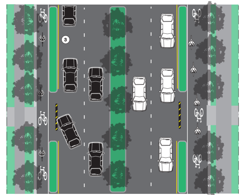
1-WAY CYCLE TRACKS ON ARTERIAL ROAD Not to scale
