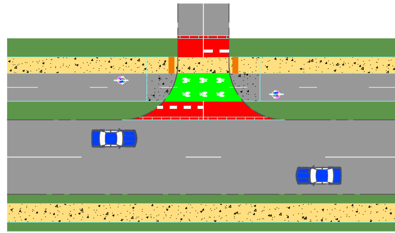
Two-way cycle track and footpath at side road (Refer below for details)
