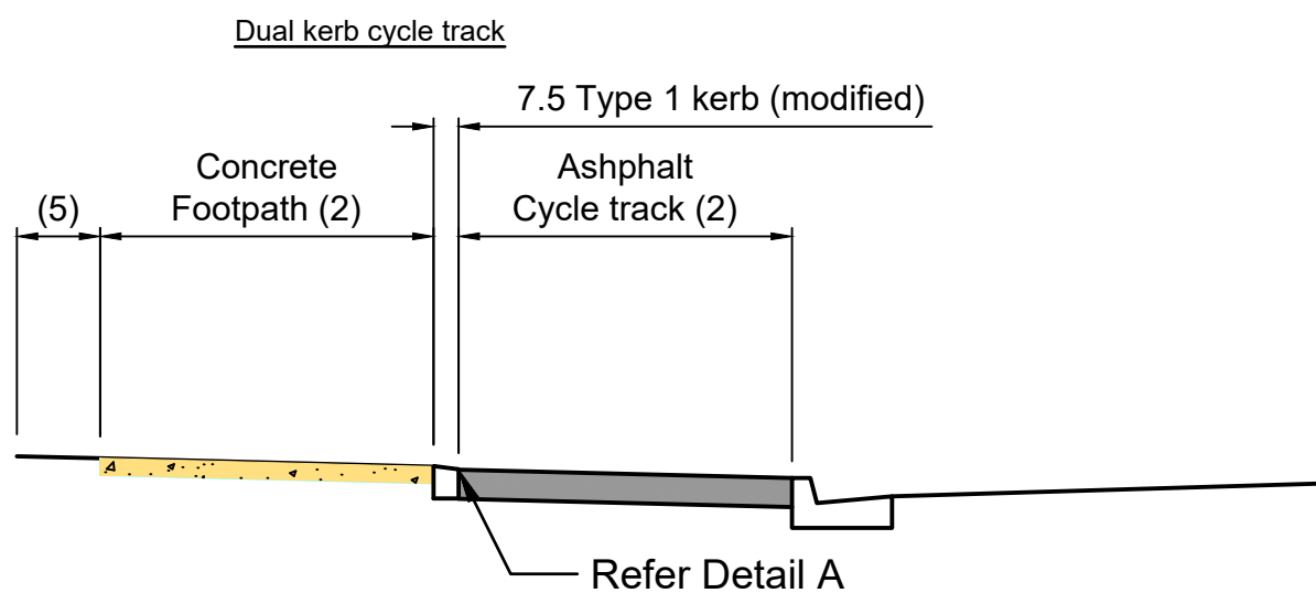
Dual kerb cycle track (constrained corridors with no parking or residential frontage)
