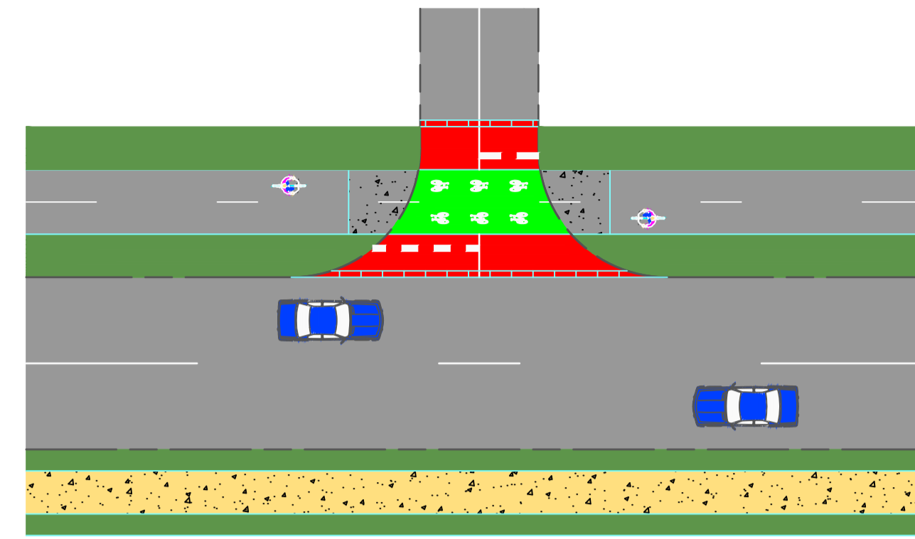
Two-way cycle track at side road
