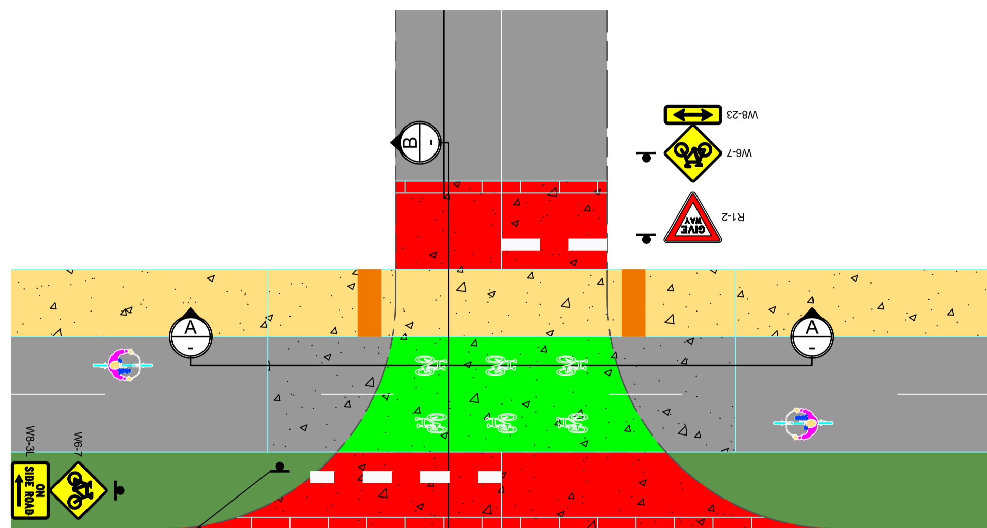
Two-way cycle track and footpath crossing details
