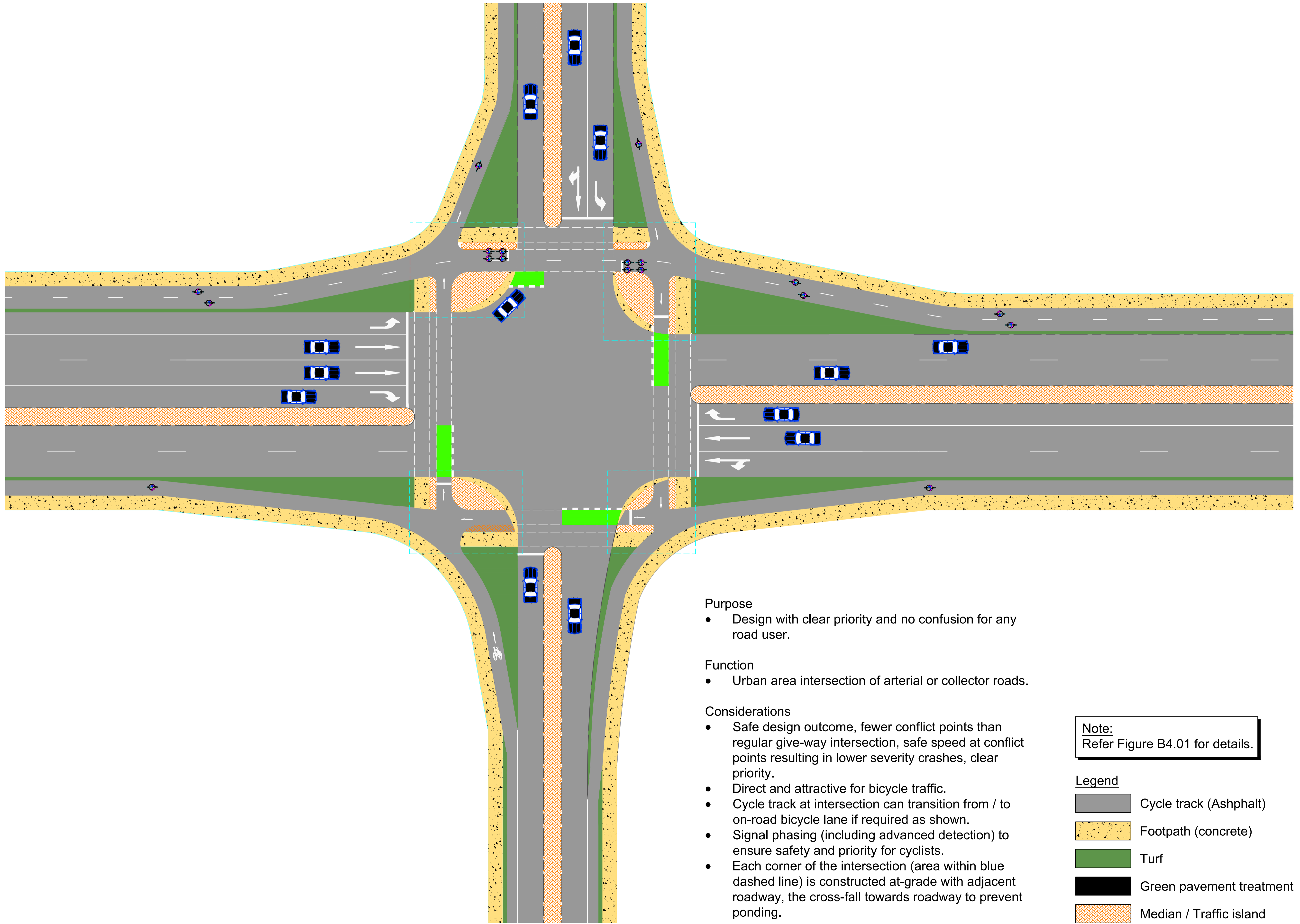
SIGNALISED 4-WAY INTERSECTION WITH ONE-WAY AND TWO-WAY CYCLE TRACKS
